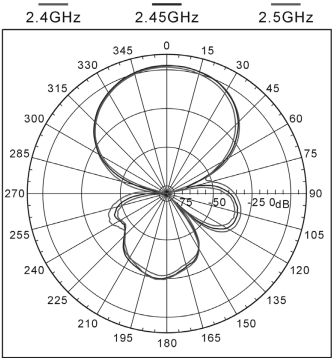
Far-field amplitude of MGA-DS-09-V-X2-4.nsi
